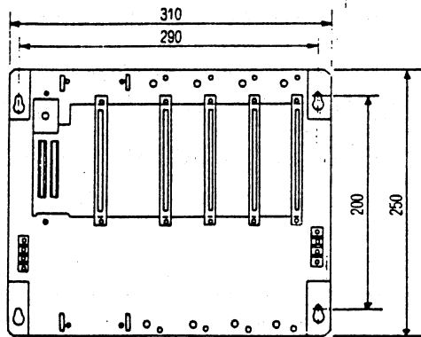
Expansion Rack Panel (ZW-104ZB)
