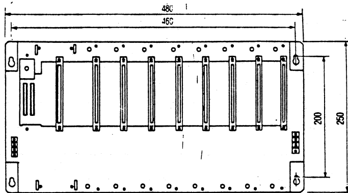
Expansion Rack Panel (ZW-108ZB)
