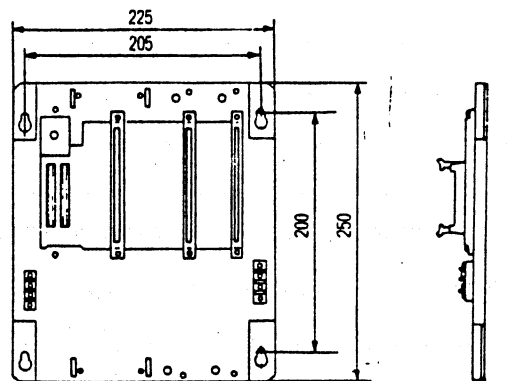
Expansion Rack Panel (ZW-102ZB)
