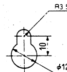
Detail of mounting hole
