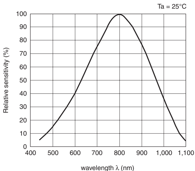
Fig. 2 Spectral Sensitivity
