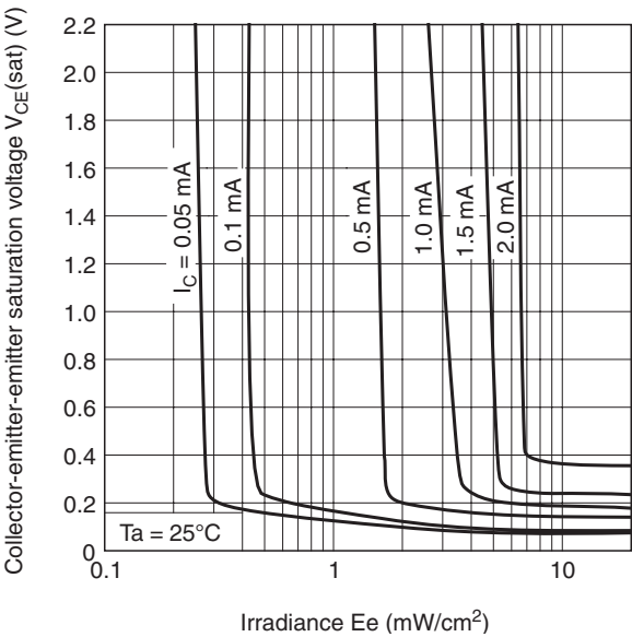
Fig. 10 Collector-to-Emitter Saturation Voltage vs. Irradiance
