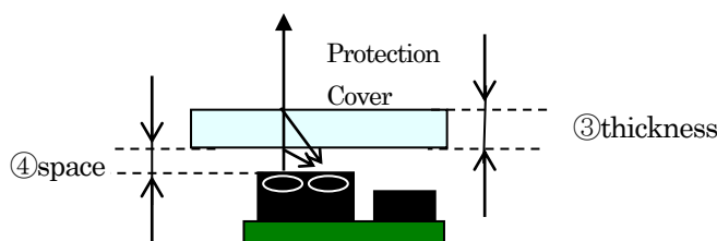
GP2Y0E02A (example)
