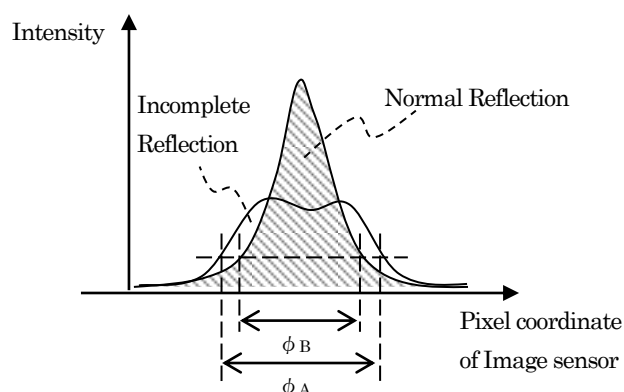
Fig.32 Spot size of incomplete and normal reflection
