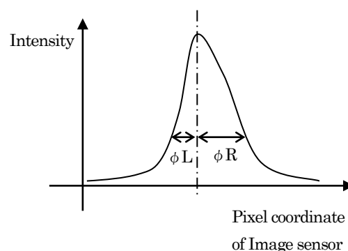
Fig.33 Asymmetric Light Spot
