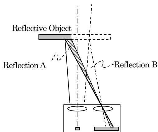
Fig.30 Partial and Whole Reflection of Emitting Beam
