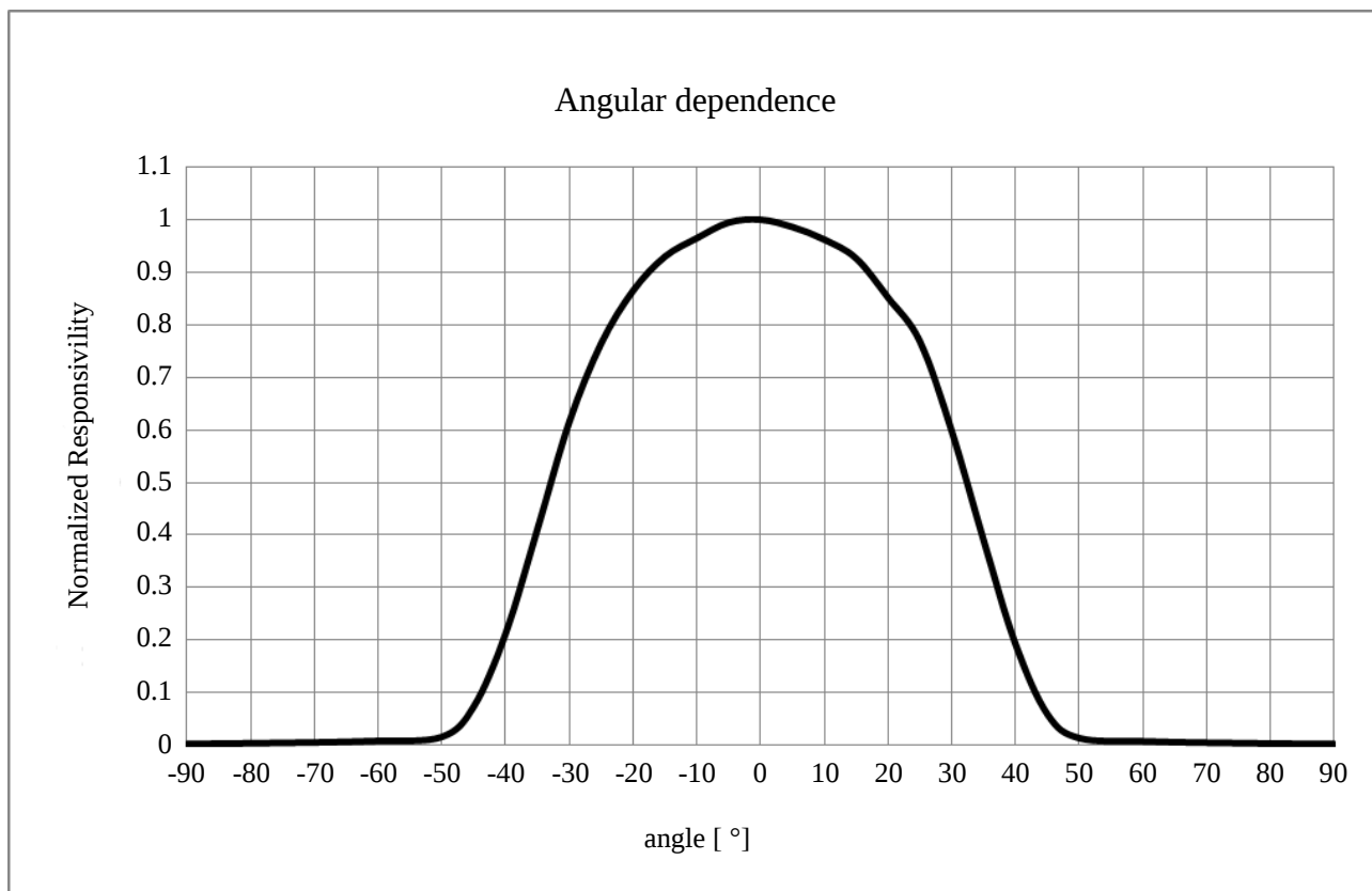
Fig.22 Angular dependence
