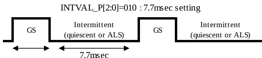
Fig.13 Intermittent operating
