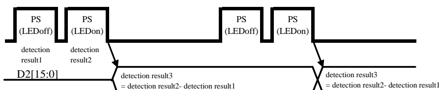
Fig.11 Sensing results output for PS mode (ALC=0)
