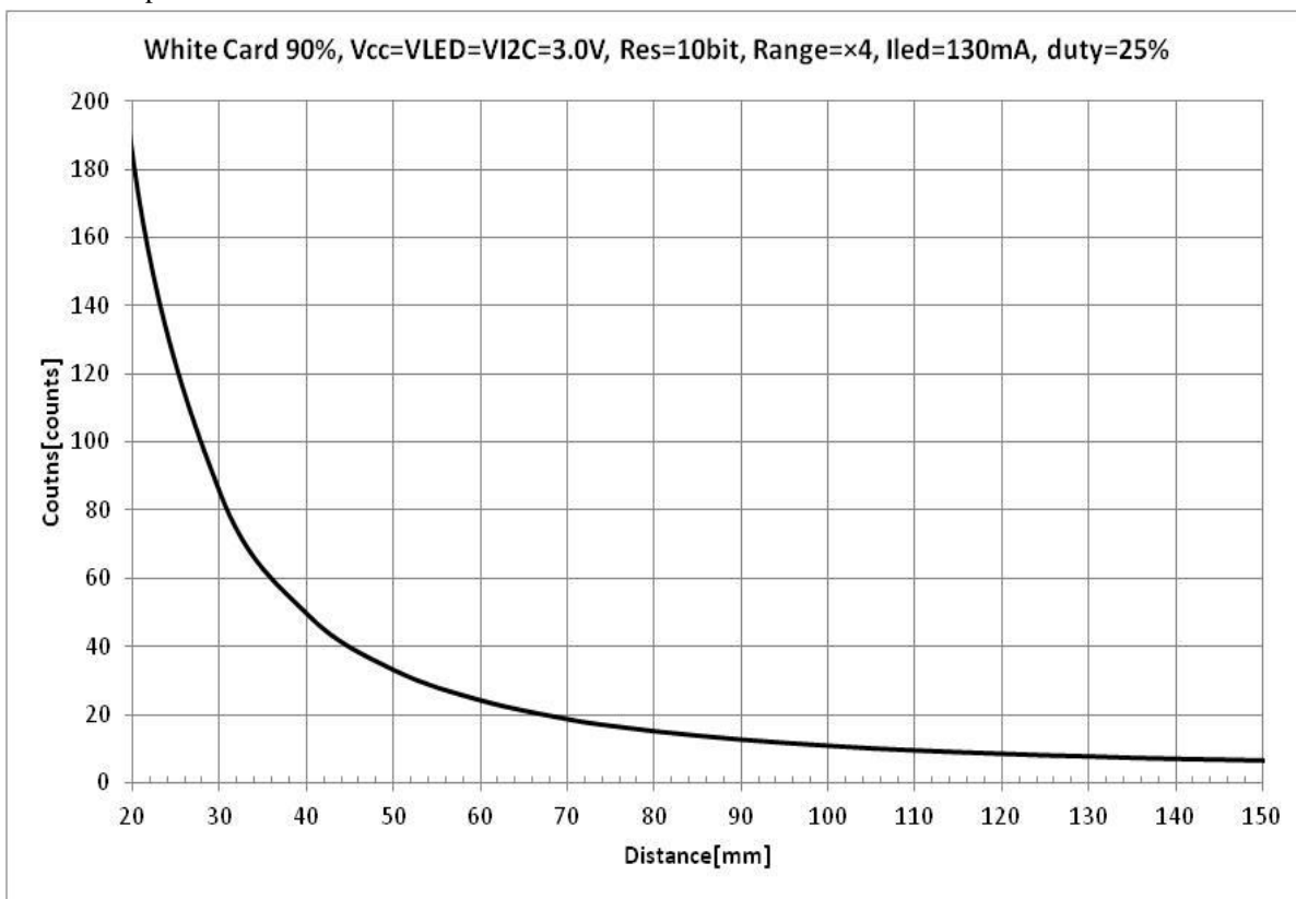
Fig.22 Sensor output counts vs. distance
