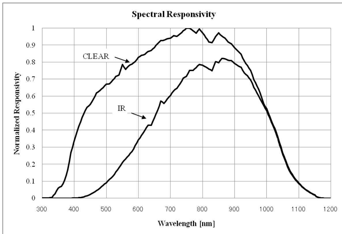
Fig.21 Spectral Responsivity
