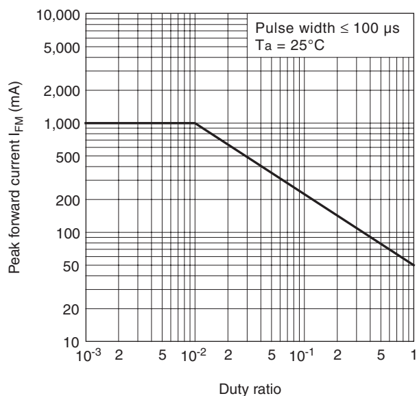
Fig. 2 Peak Forward Current vs. Duty Ratio
