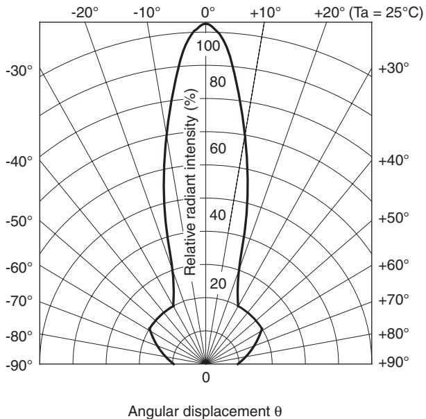
Fig. 10 Radiation Diagram
