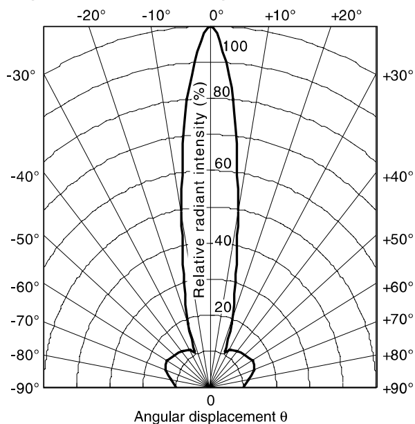
Fig. 9 Radiation Diagram
